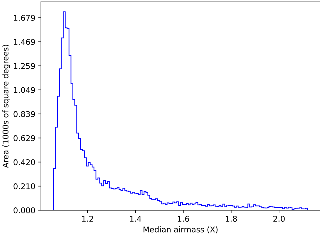
ddf_acor_sf10_lsf40_lsr20_v3.4_10yrs Yr 1 i band: Median airmass
