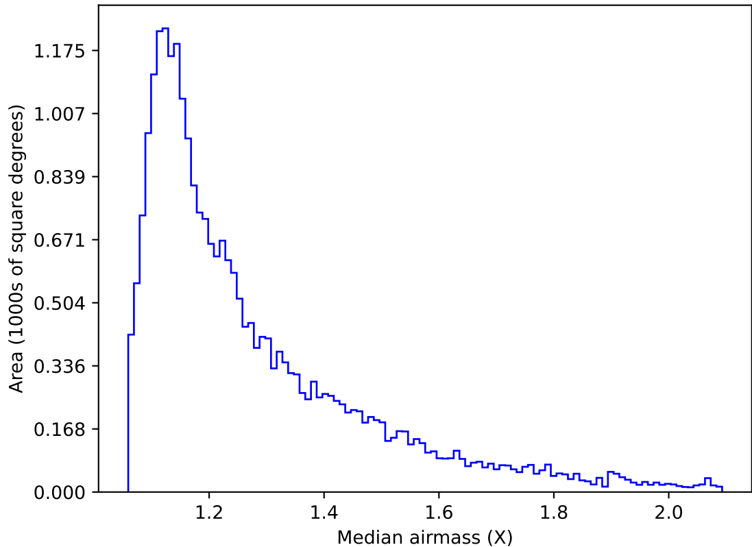
ddf_acor_sf10_lsf40_lsr20_v3.4_10yrs Yr 1 g band: Median airmass
