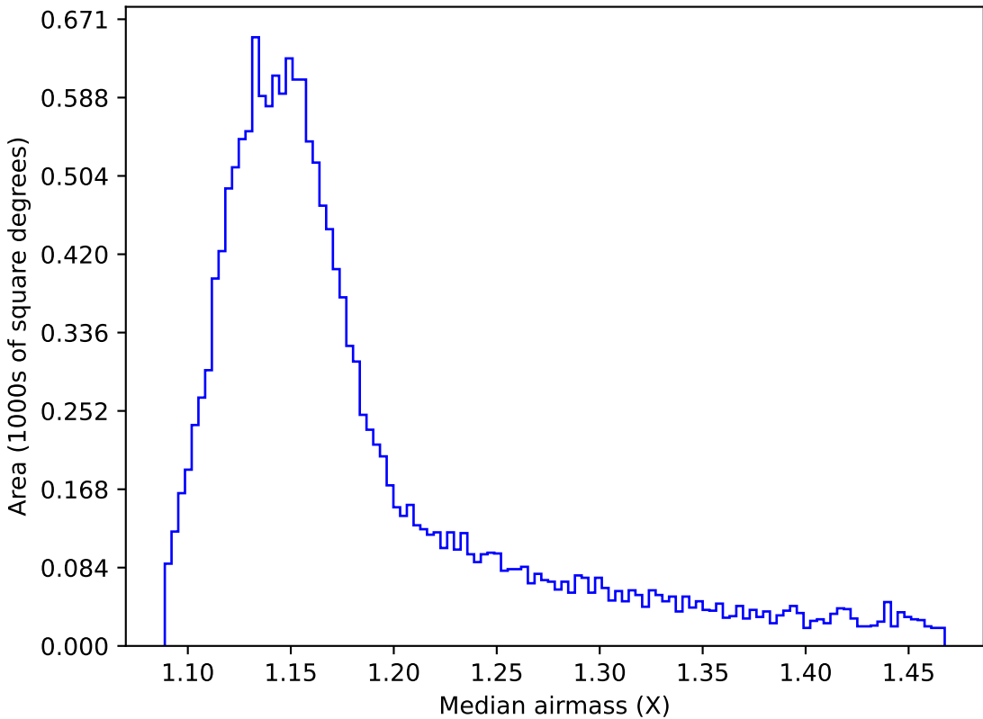
ddf_acor_sf10_lsf40_lsr20_v3.4_10yrs WFD z band: Median airmass
