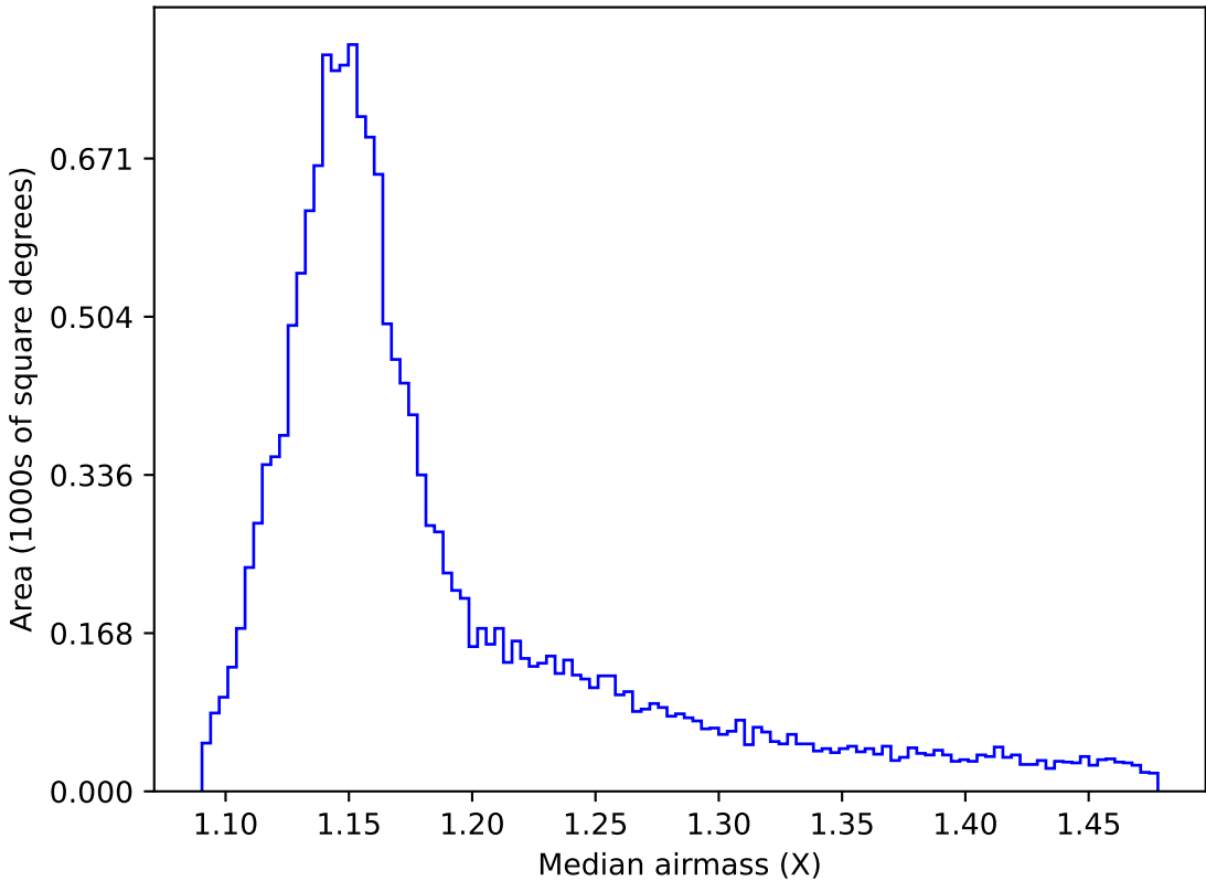
ddf_acor_sf10_ls40_lsr20_v3.4_10yrs WFD y band: Median airmass
