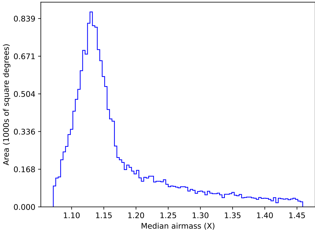
ddf_acor_sf10_lsf40_lsr20_v3.4_10yrs WFD r band: Median airmass
