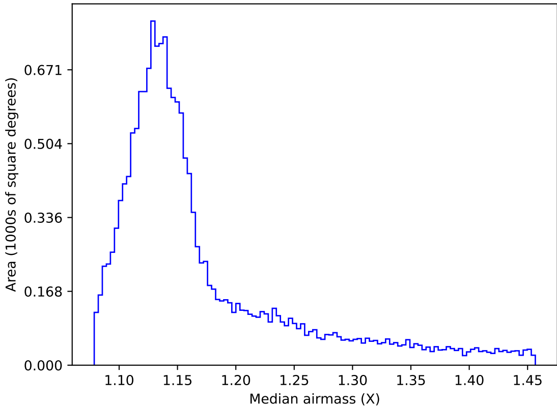
ddf_acor_sf10_lsf40_lsr20_v3.4_10yrs WFD i band: Median airmass
