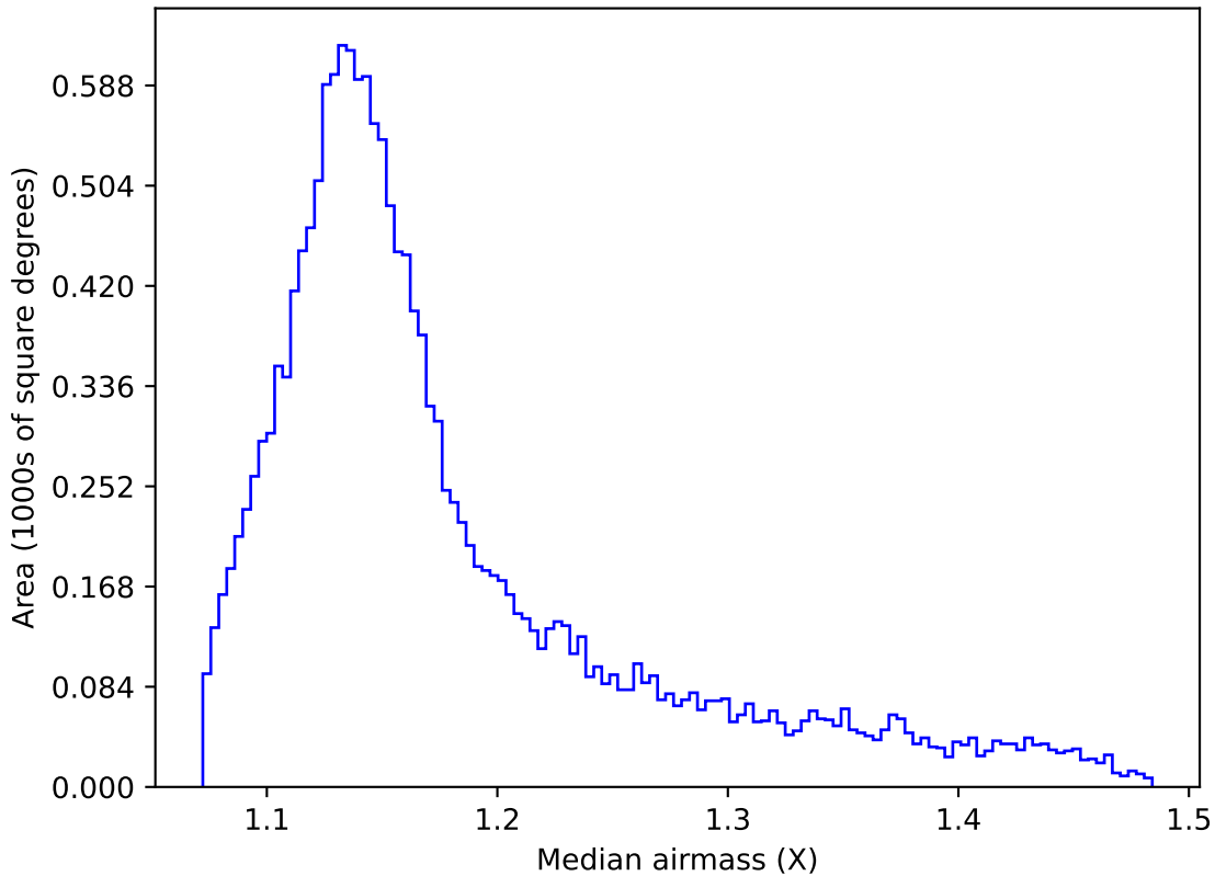
ddf_acor_sf10_lsf40_lsr20_v3.4_10yrs WFD g band: Median airmass
