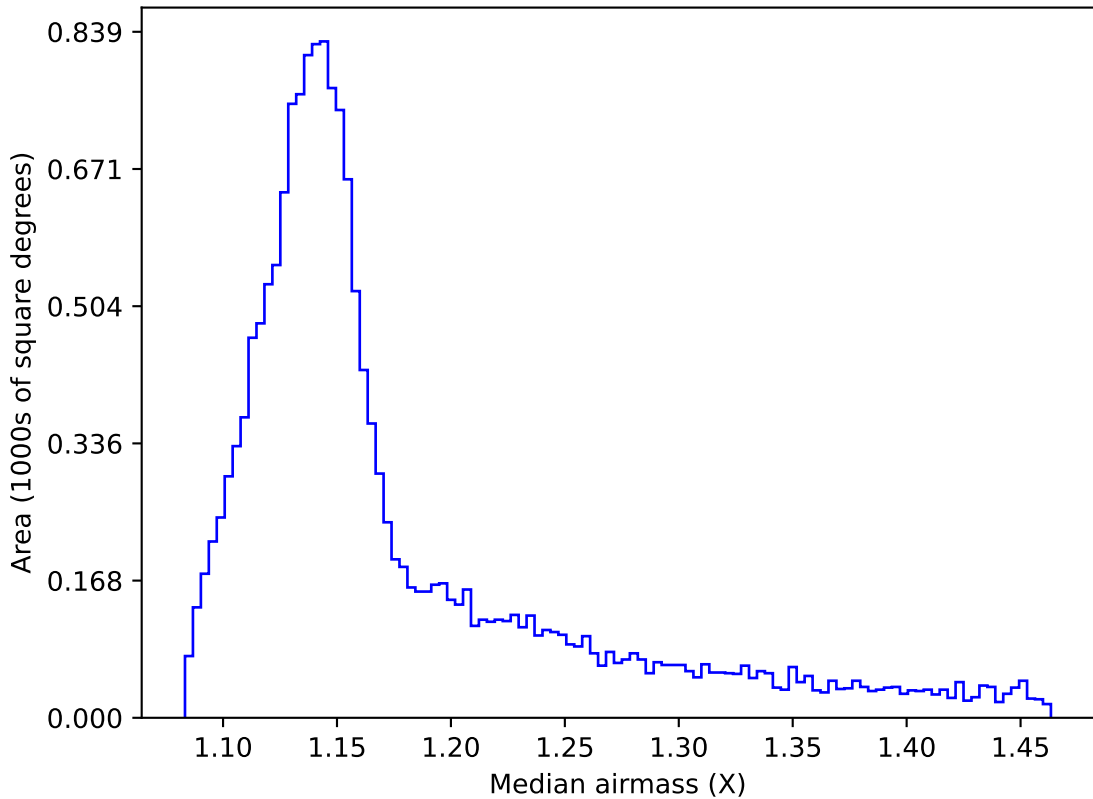
ddf_acor_sf10_lsf40_lsr20_v3.4_10yrs WFD all bands: Median airmass
