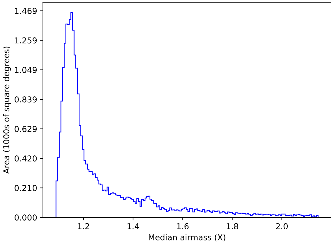
ddf_acor_sf10_lsf40_lsr20_v3.4_10yrs All sky z band: Median airmass
