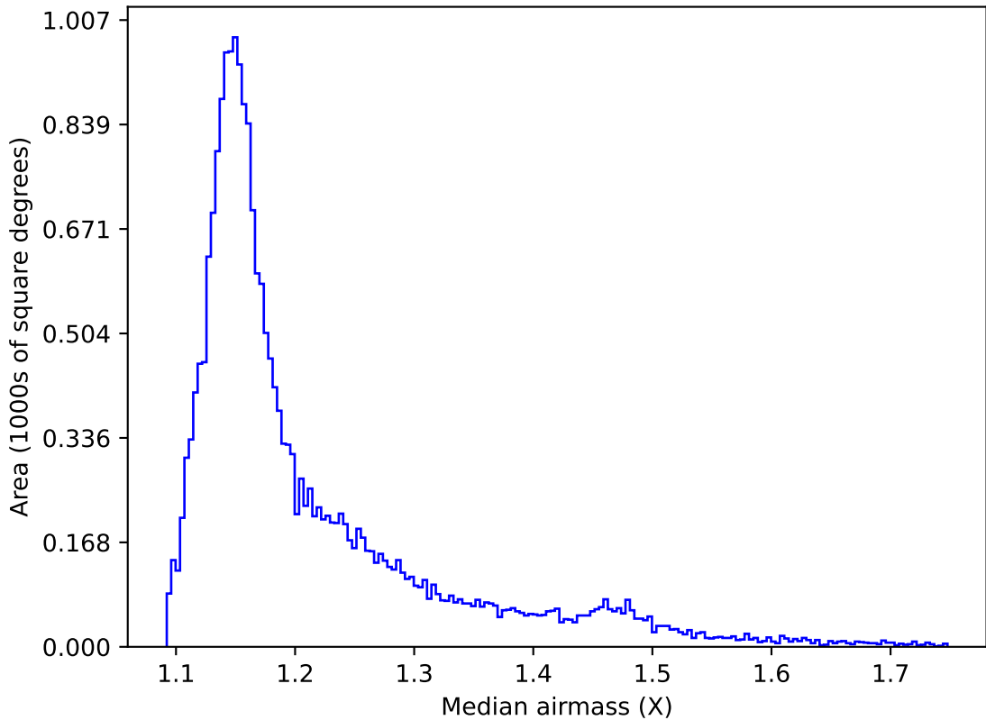
ddf_acor_sf10_lsf40_lsr20_v3.4_10yrs All sky y band: Median airmass
