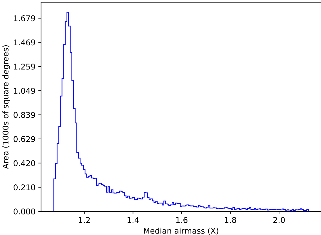
ddf_acor_sf10_lsf40_lsr20_v3.4_10yrs All sky r band: Median airmass
