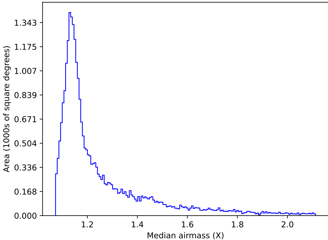
ddf_acor_sf10_lsf40_lsr20_v3.4_10yrs All sky g band: Median airmass
