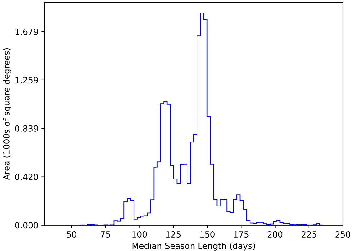
ddf_acor_sf10_lsf40_lsr20_v3.4_10yrs WFD y band: Median Season Length
