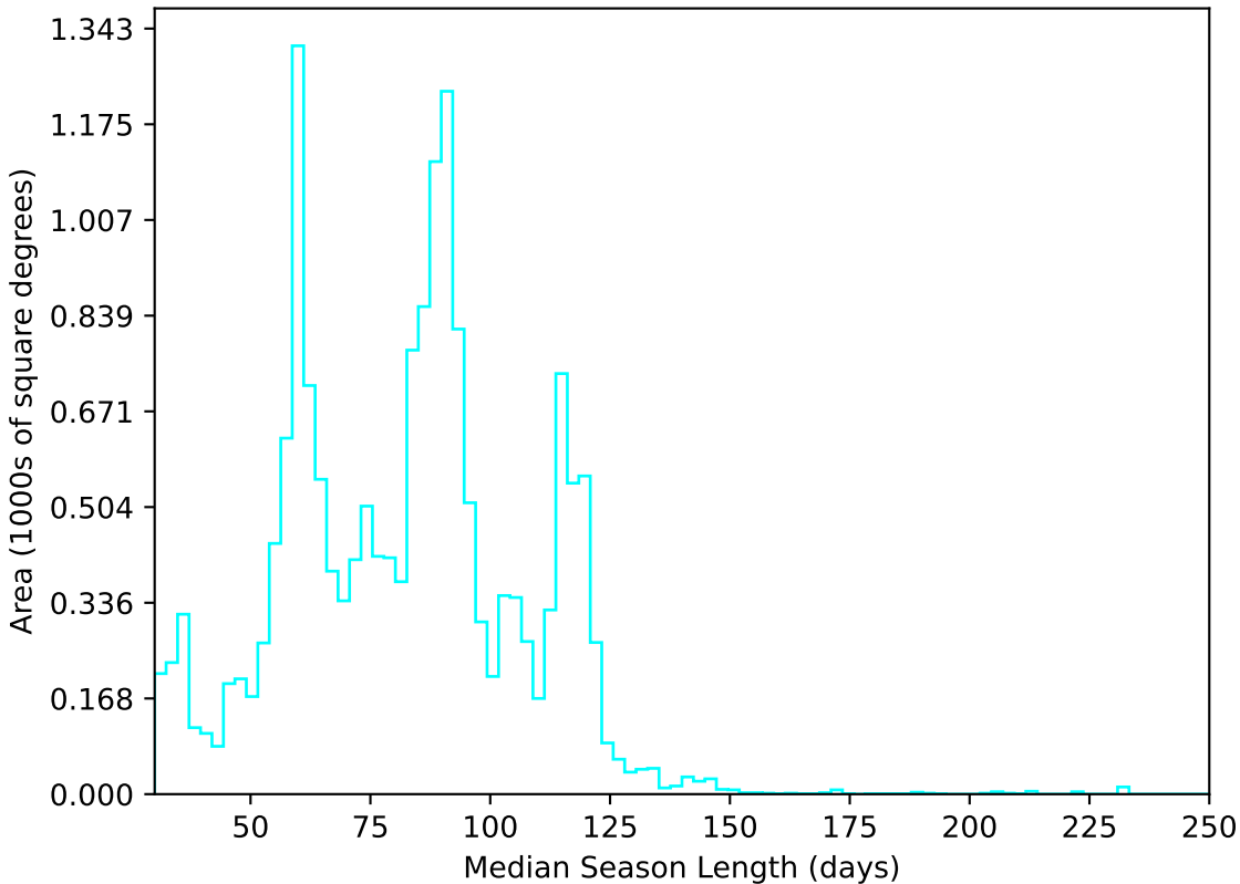
ddf_acor_sf10_lsf40_lsr20_v3.4_10yrs WFD u band: Median Season Length
