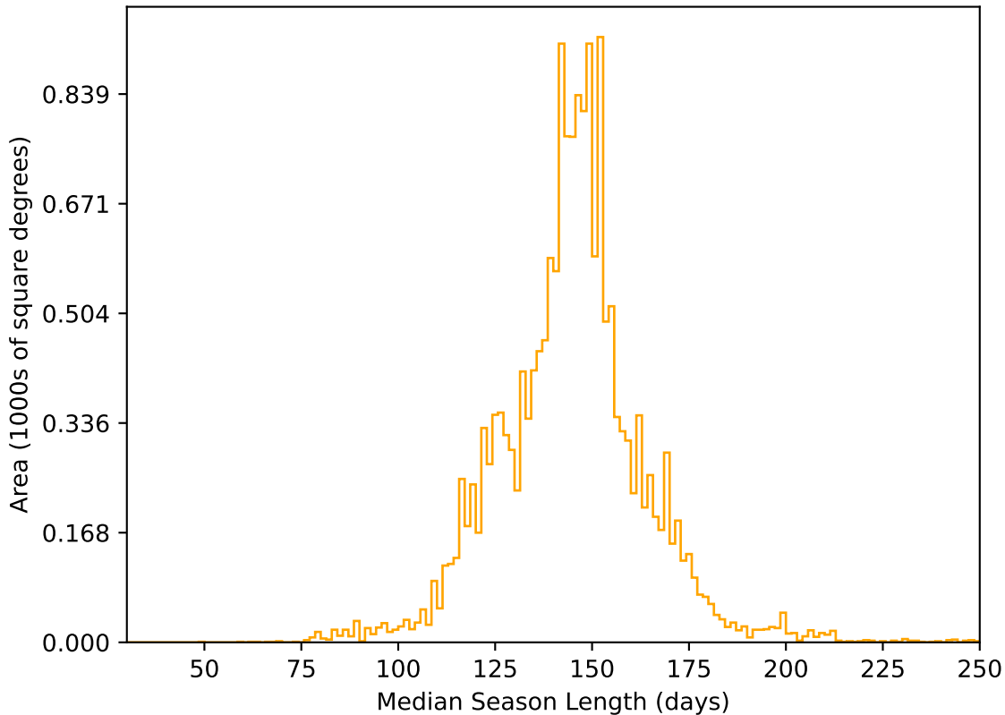
ddf_acor_sf10_lsf40_lsr20_v3.4_10yrs WFD r band: Median Season Length
