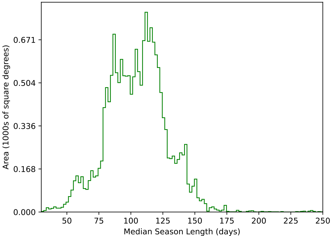
ddf_acor_sf10_ls40_lsr20_v3.4_10yrs WFD g band: Median Season Length
