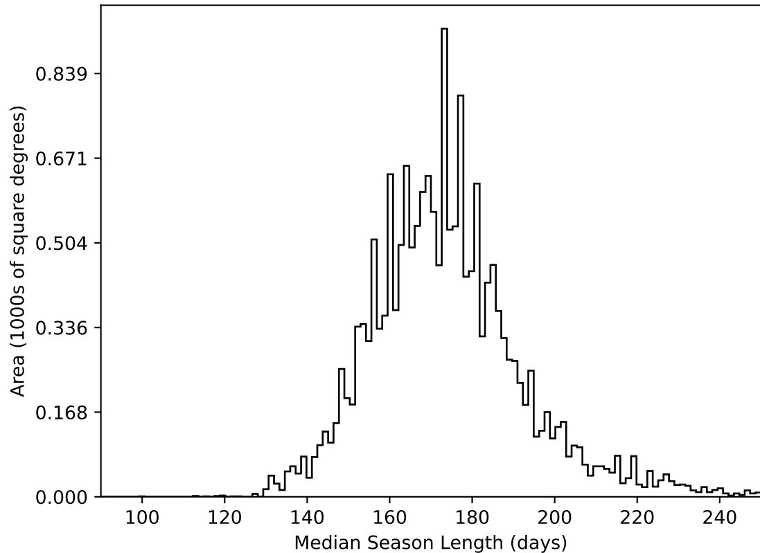
ddf_acor_sf10_lsf40_lsr20_v3.4_10yrs WFD all bands: Median Season Length
