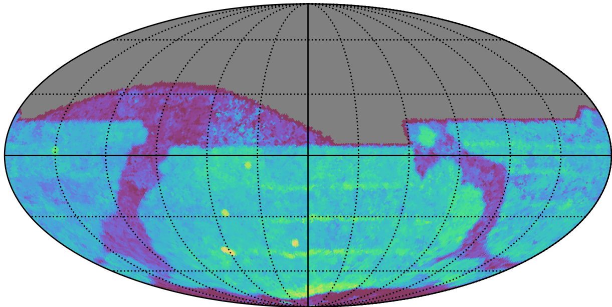
ddf_acor_sf10_lsf40_lsr20_v3.4_10yrs All sky z band: Median Season Length
