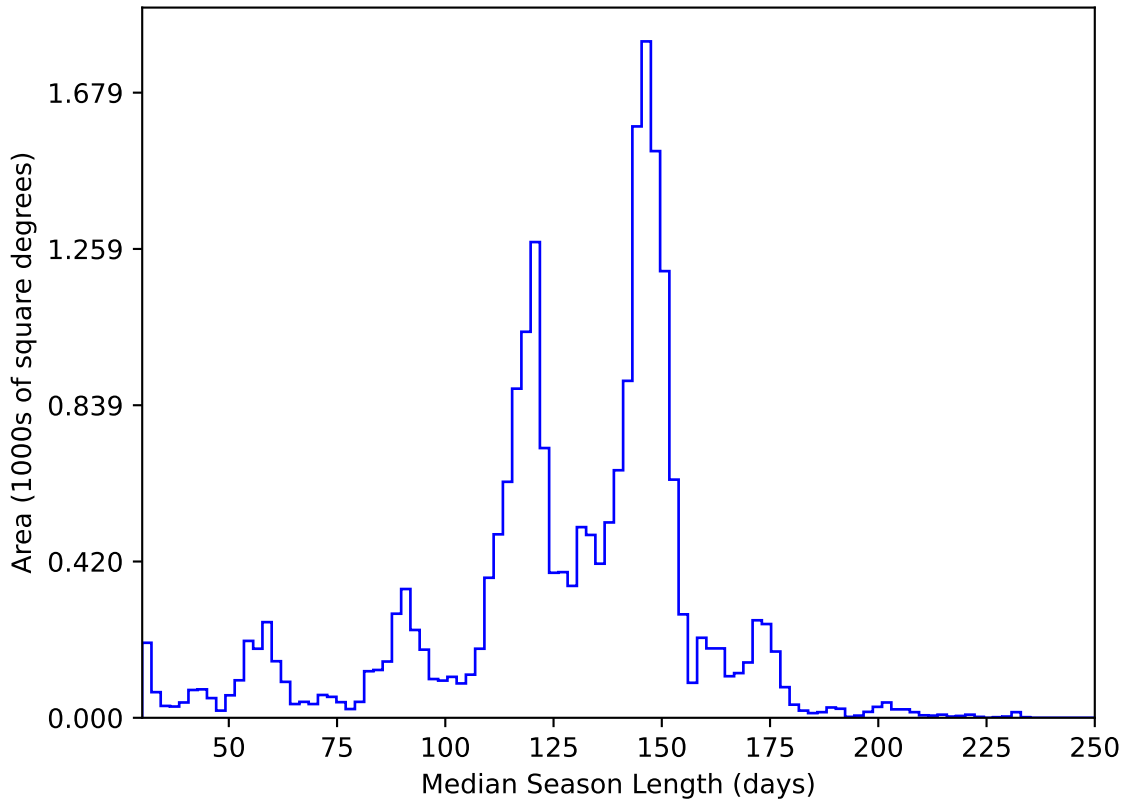
ddf_acor_sf10_lsf40_lsr20_v3.4_10yrs All sky y band: Median Season Length
