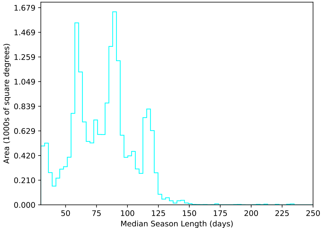
ddf_acor_sf10_lsf40_lsr20_v3.4_10yrs All sky u band: Median Season Length
