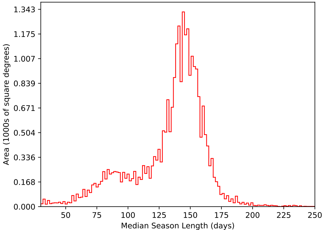
ddf_acor_sf10_Isf40_Isr20_v3.4_10yrs All sky i band: Median Season Length
