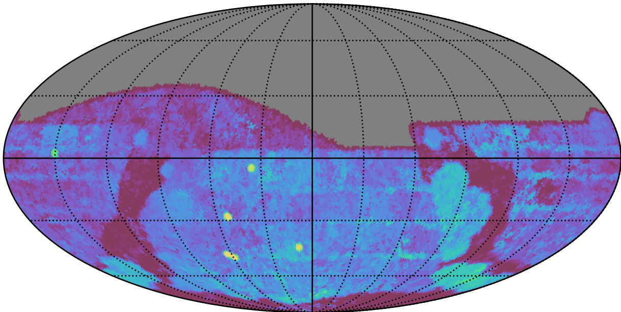
ddf_acor_sf10_lsf40_lsr20_v3.4_10yrs All sky g band: Median Season Length
