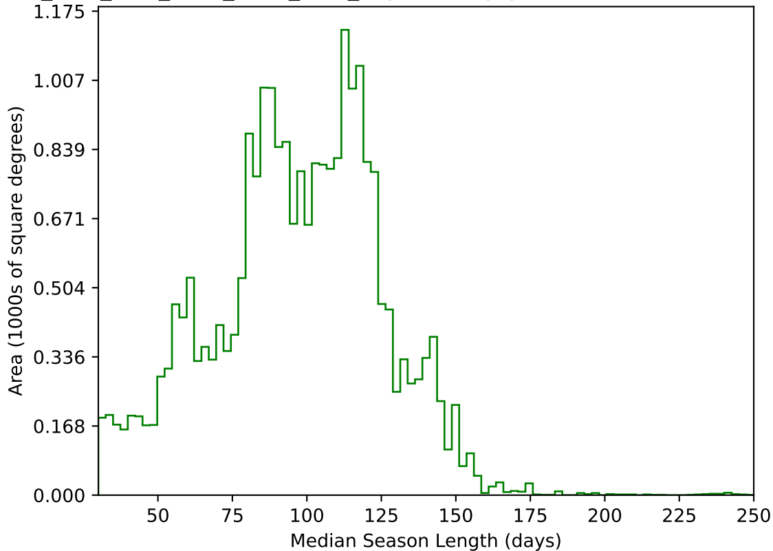
ddf_acor_sf10_lsf40_lsr20_v3.4_10yrs All sky g band: Median Season Length
