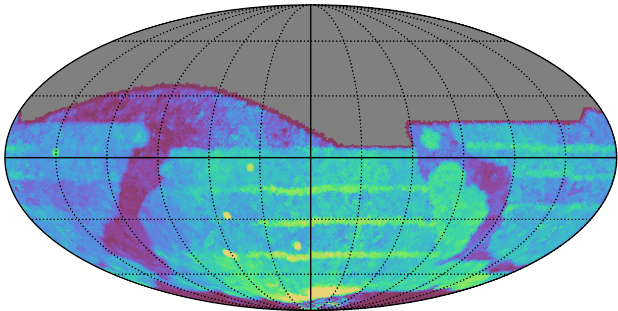
ddf_acor_sf10_lsf40_lsr20_v3.4_10yrs All sky all bands: Median Season Length
