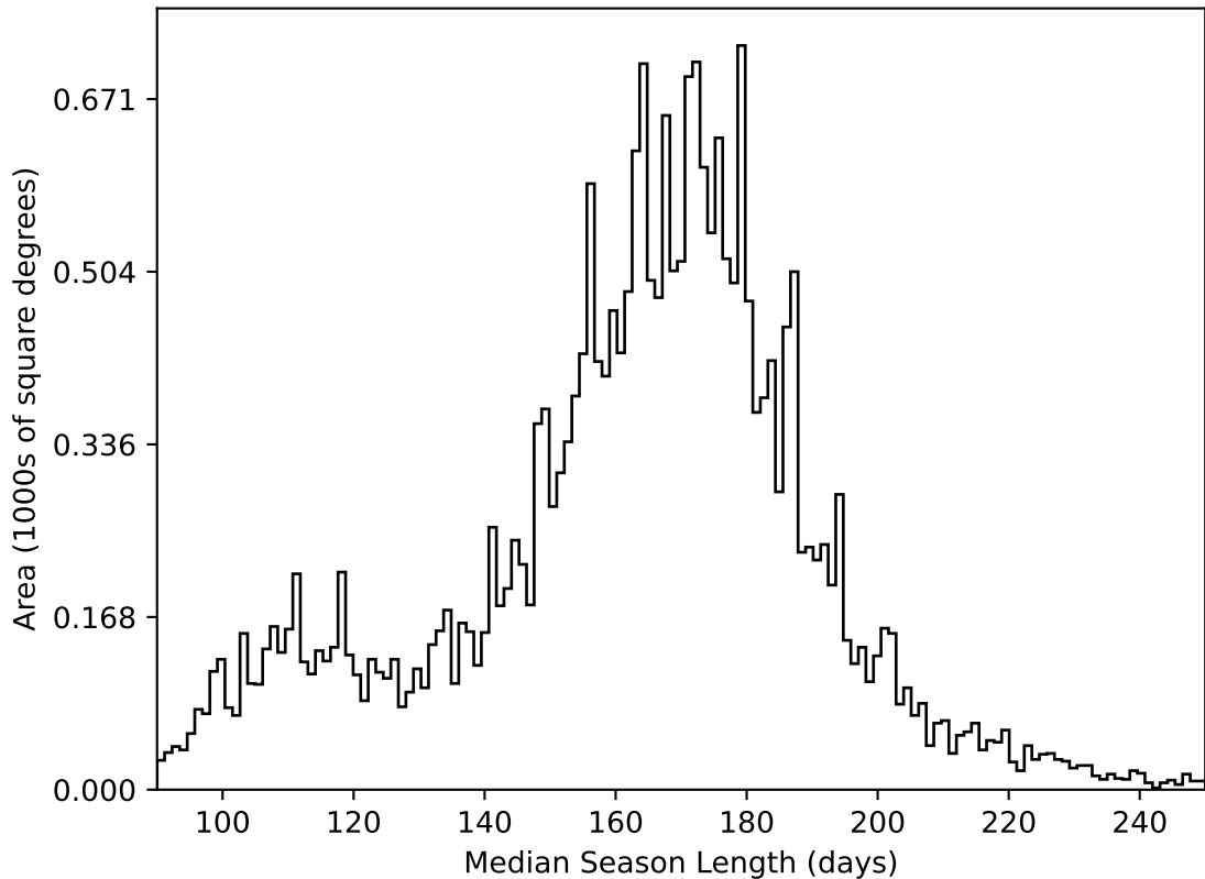
ddf_acor_sf10_lsf40_lsr20_v3.4_10yrs All sky all bands: Median Season Length
