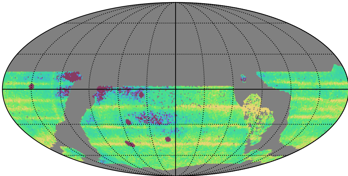
ddf_acor_sf10_lsf40_lsr20_v3.4_10yrs WFD: Median Intra-Night Gap
