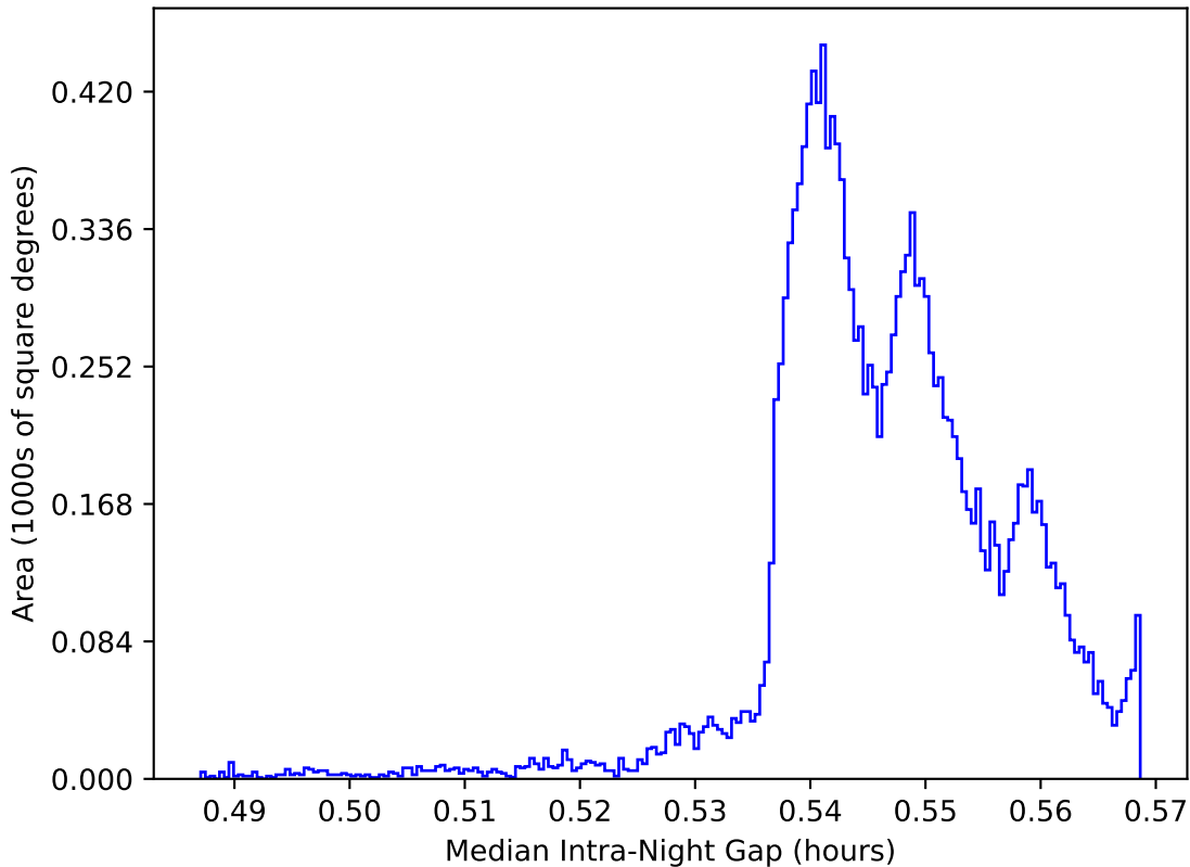
ddf_acor_sf10_lsf40_lsr20_v3.4_10yrs WFD: Median Intra-Night Gap
