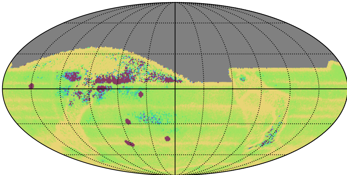
ddf_acor_sf10_lsf40_lsr20_v3.4_10yrs All sky: Median Intra-Night Gap
