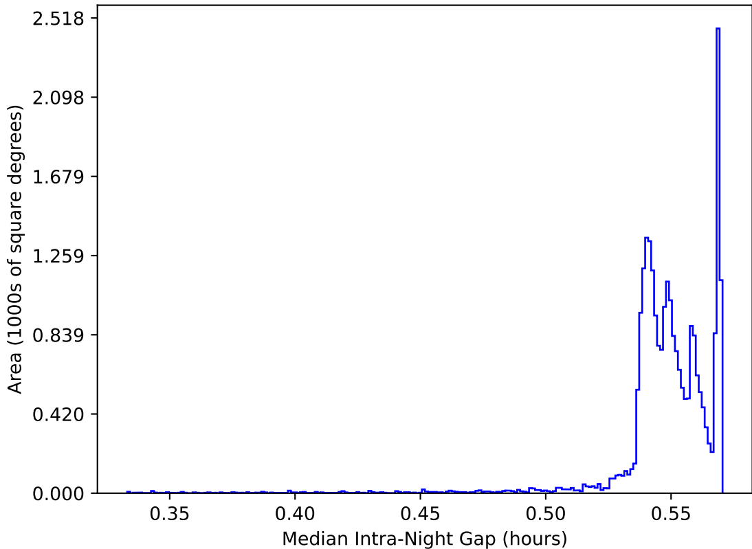
ddf_acor_sf10_lsf40_lsr20_v3.4_10yrs All sky: Median Intra-Night Gap
