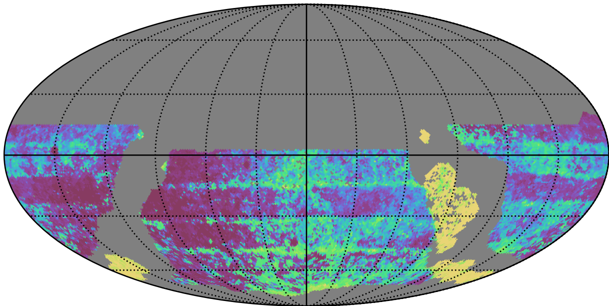
ddf_acor_sf10_lsf40_lsr20_v3.4_10yrs WFD y band: Median Inter-Night Gap
