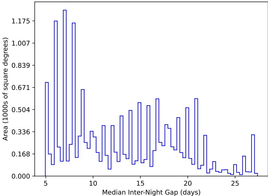
ddf_acor_sf10_lsf40_lsr20_v3.4_10yrs WFD y band: Median Inter-Night Gap
