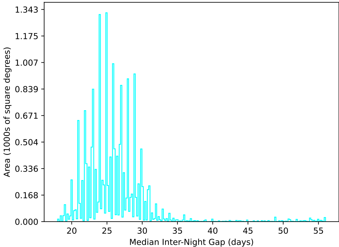
ddf_acor_sf10_lsf40_lsr20_v3.4_10yrs WFD u band: Median Inter-Night Gap
