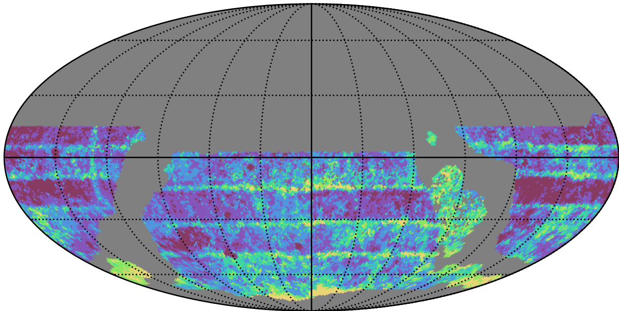
ddf_acor_sf10_lsf40_lsr20_v3.4_10yrs WFD r band: Median Inter-Night Gap
