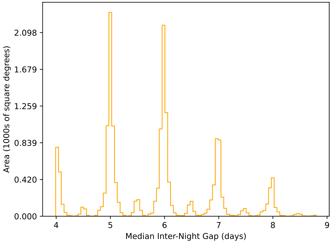
ddf_acor_sf10_lsf40_lsr20_v3.4_10yrs WFD r band: Median Inter-Night Gap
