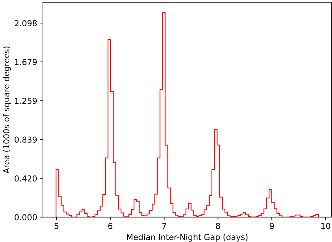
ddf_acor_sf10_lsf40_lsr20_v3.4_10yrs WFD i band: Median Inter-Night Gap
