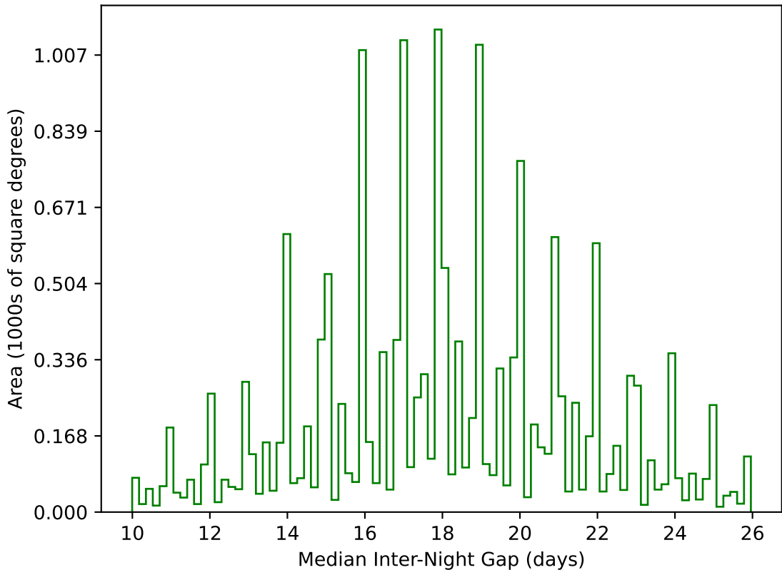
ddf_acor_sf10_lsf40_lsr20_v3.4_10yrs WFD g band: Median Inter-Night Gap
