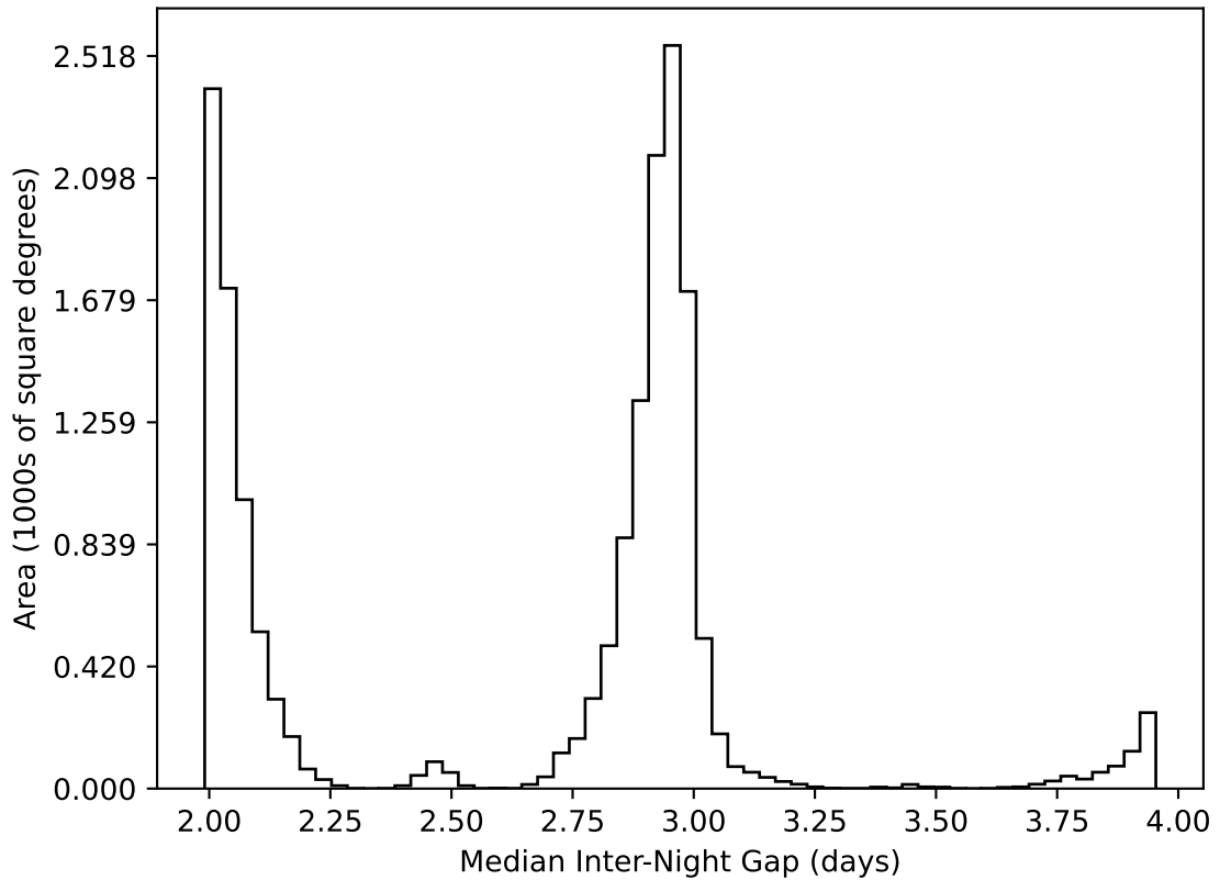
ddf_acor_sf10_lsf40_lsr20_v3.4_10yrs WFD all bands: Median Inter-Night Gap
