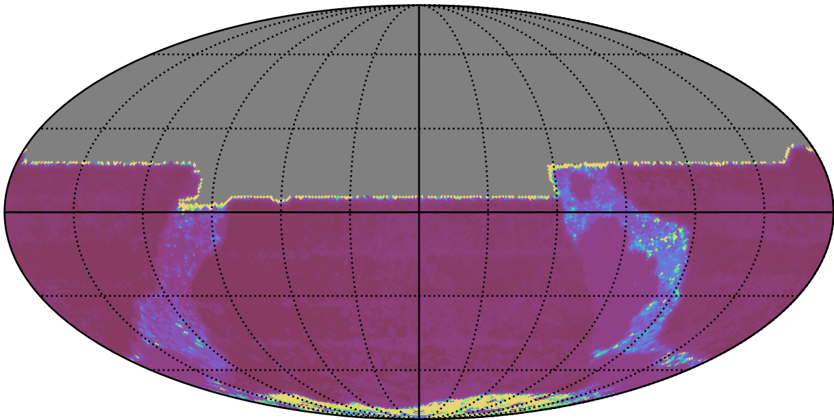
ddf_acor_sf10_lsf40_lsr20_v3.4_10yrs All sky y band: Median Inter-Night Gap
