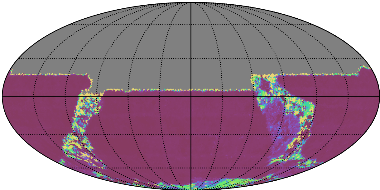
ddf_acor_sf10_lsf40_lsr20_v3.4_10yrs All sky u band: Median Inter-Night Gap
