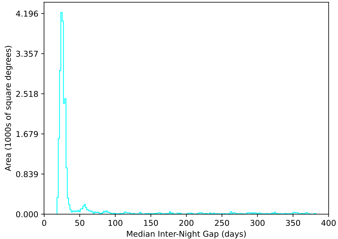
ddf_acor_sf10_lsf40_lsr20_v3.4_10yrs All sky u band: Median Inter-Night Gap
