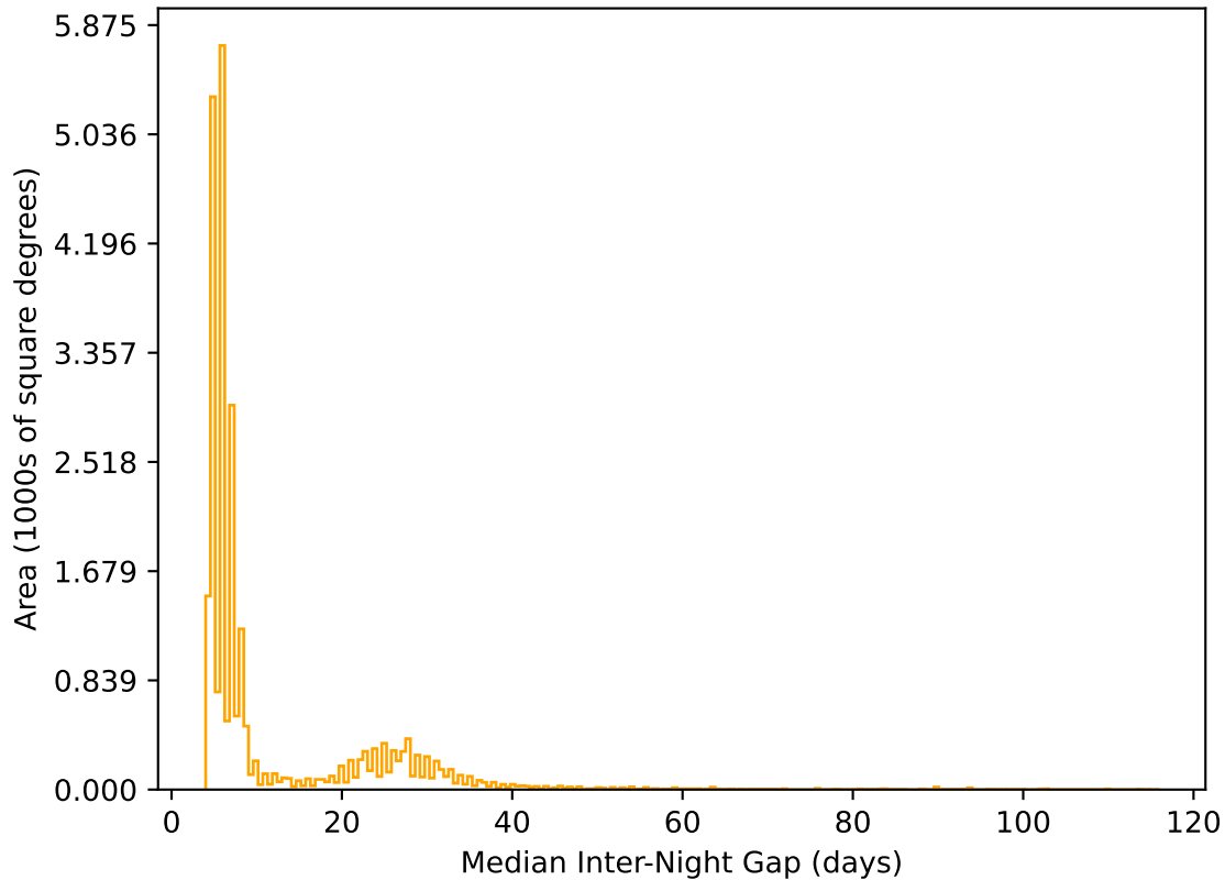
ddf_acor_sf10_lsf40_lsr20_v3.4_10yrs All sky r band: Median Inter-Night Gap
