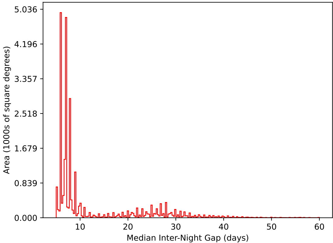
ddf_acor_sf10_lsf40_lsr20_v3.4_10yrs All sky i band: Median Inter-Night Gap
