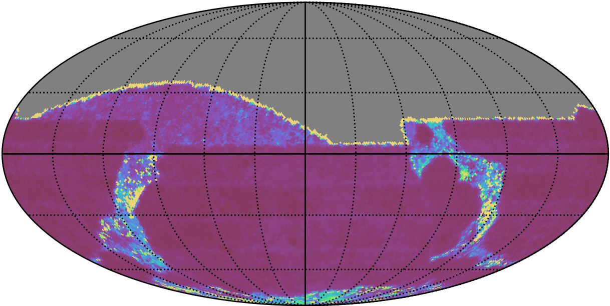
ddf_acor_sf10_lsf40_lsr20_v3.4_10yrs All sky g band: Median Inter-Night Gap
