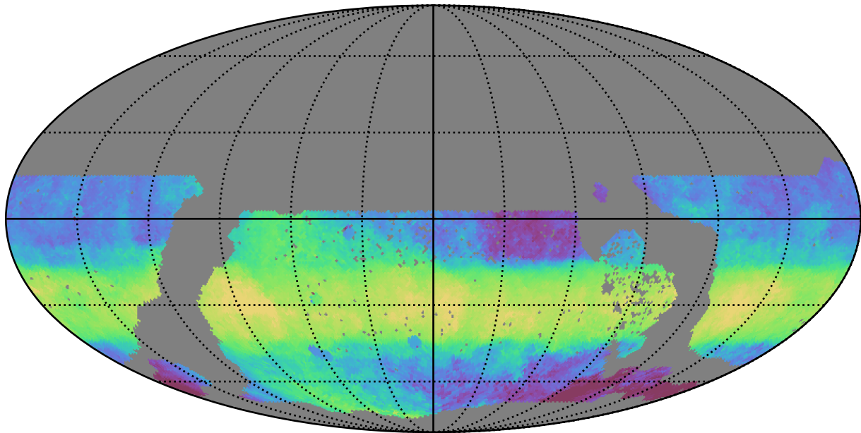
ddf_acor_sf10_lsf40_lsr20_v3.4_10yrs WFD z band: Median HA
