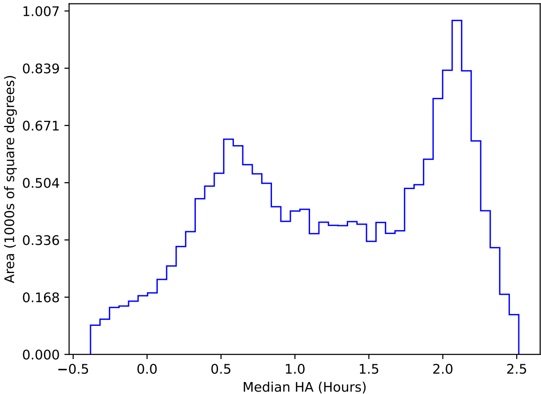
ddf_acor_sf10_lsf40_lsr20_v3.4_10yrs WFD y band: Median HA
