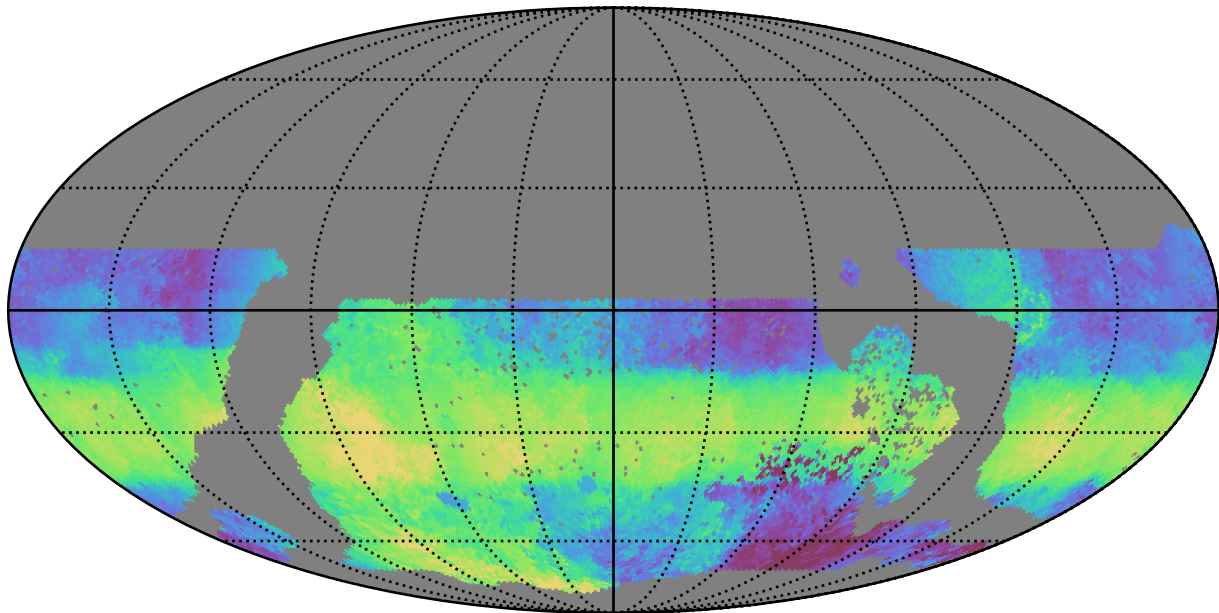
ddf_acor_sf10_lsf40_lsr20_v3.4_10yrs WFD u band: Median HA
