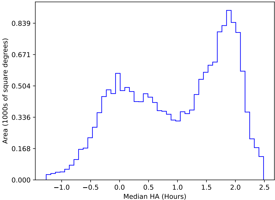
ddf_acor_sf10_lsf40_lsr20_v3.4_10yrs WFD u band: Median HA
