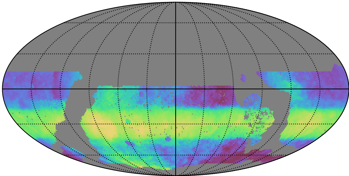
ddf_acor_sf10_lsf40_lsr20_v3.4_10yrs WFD r band: Median HA
