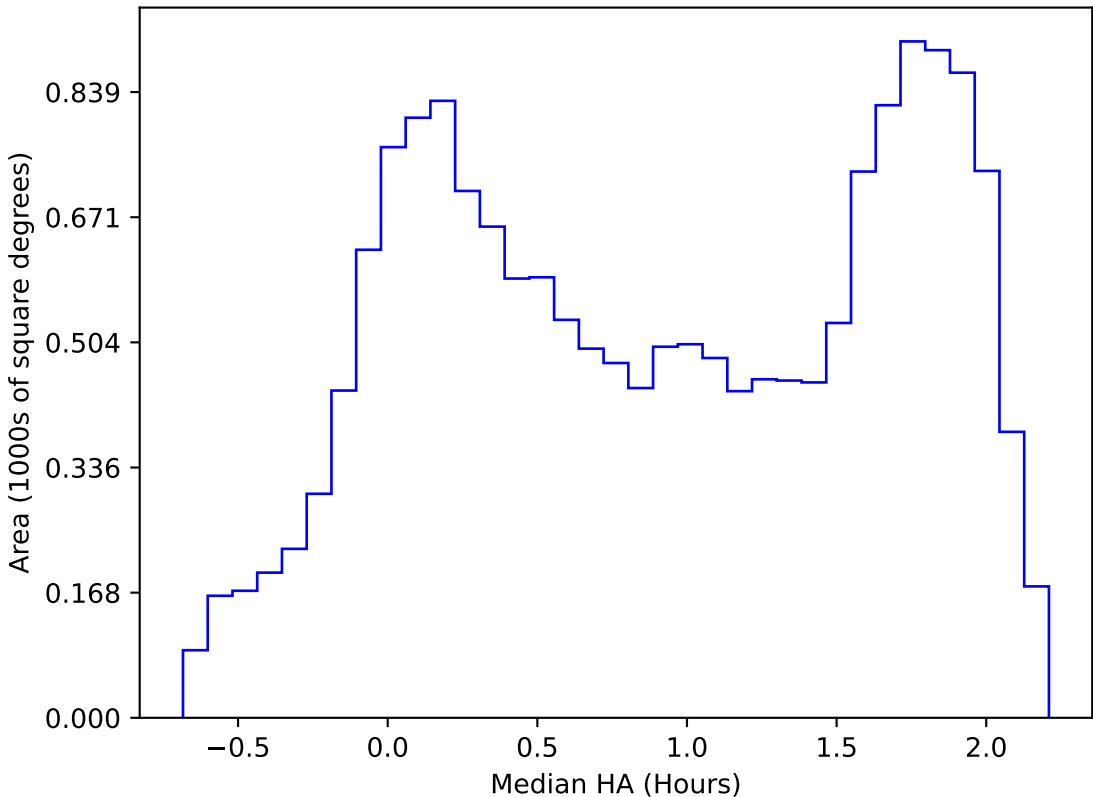
ddf_acor_sf10_lsf40_lsr20_v3.4_10yrs WFD r band: Median HA
