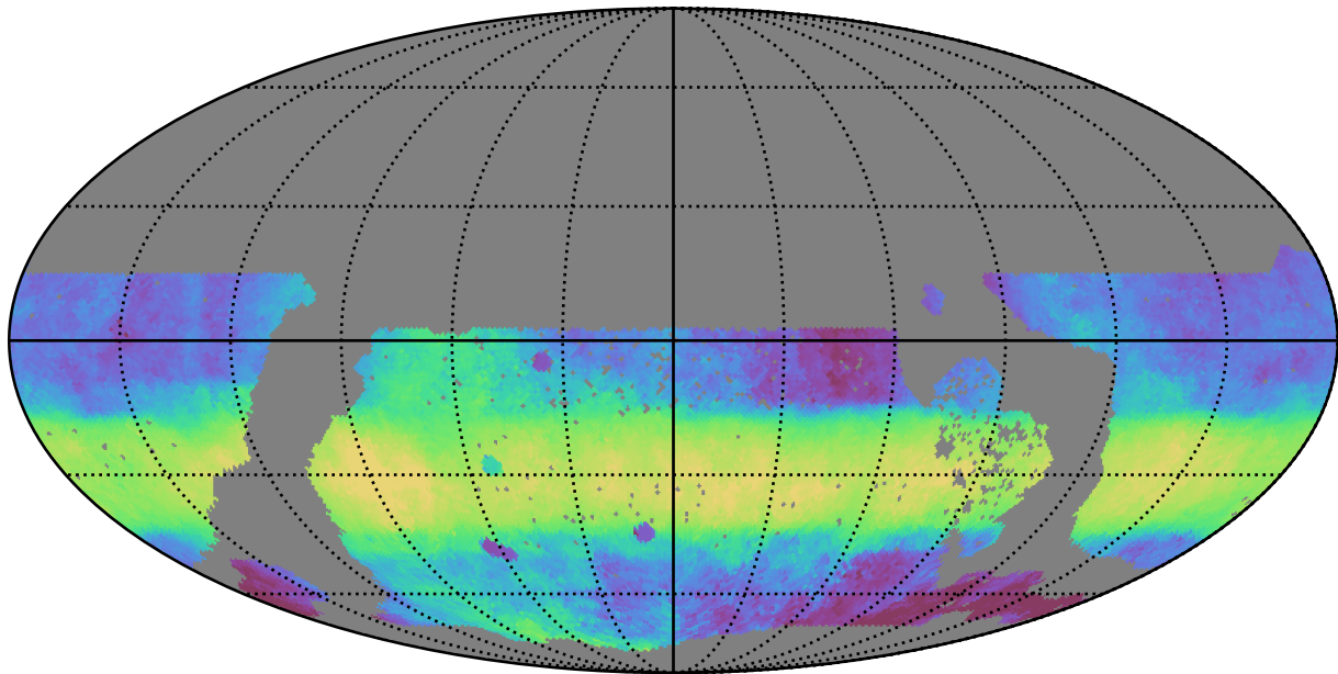
ddf_acor_sf10_lsf40_lsr20_v3.4_10yrs WFD i band: Median HA
